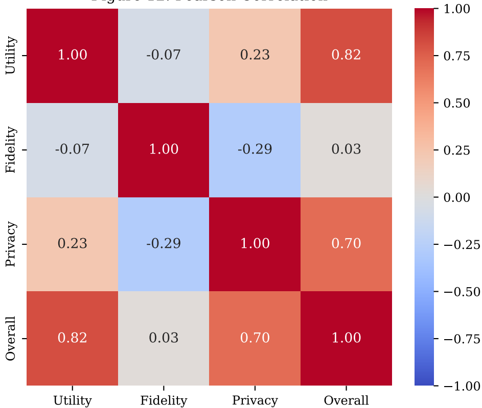
Figure 12: Pearson Correlation
