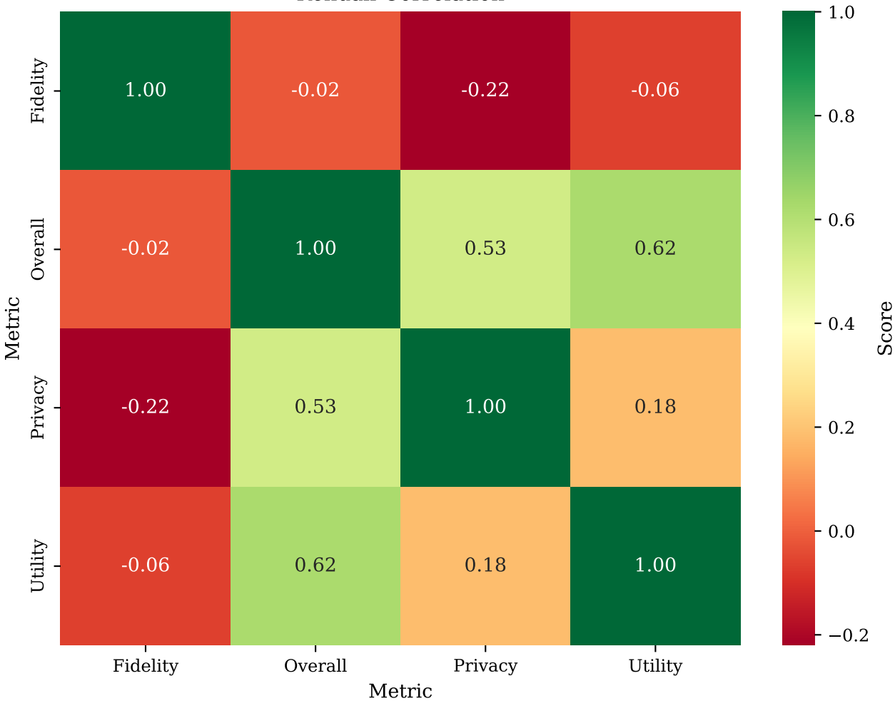
Kendall Correlation
