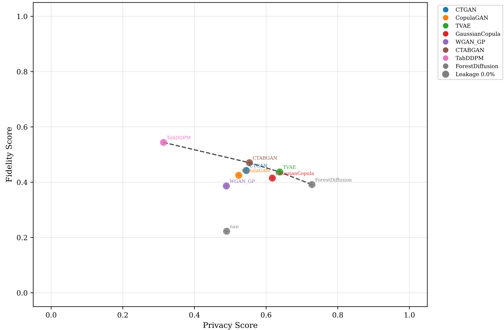
Figure 3: Privacy vs Fidelity
