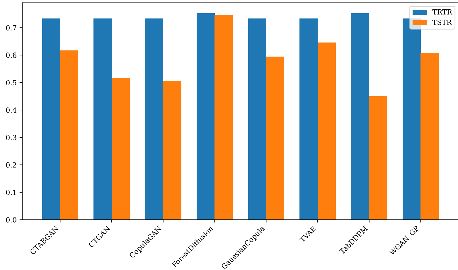
Figure 9: TRTR vs TSTR (F1)
