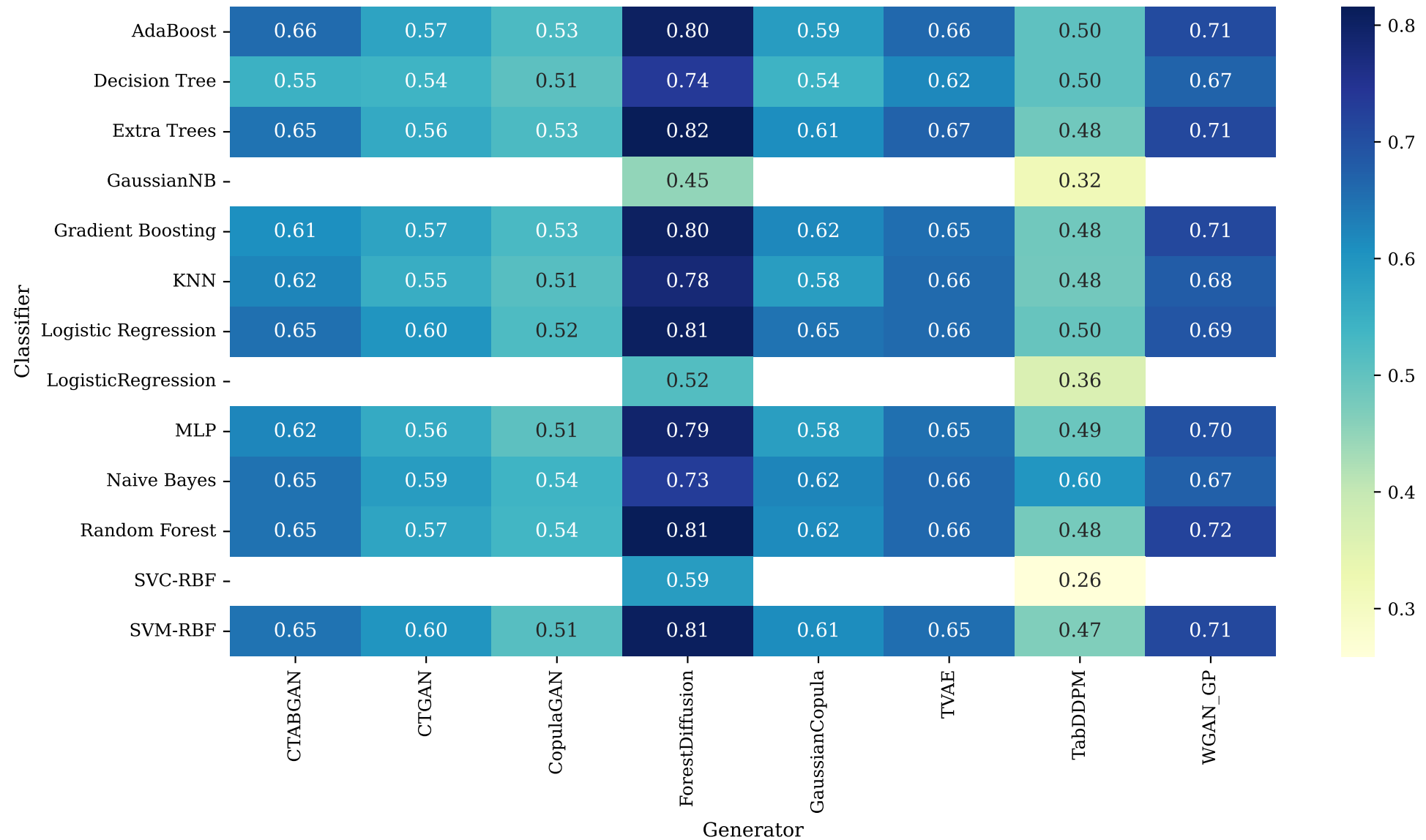
Figure 10: Precision by Classifier × Generator
