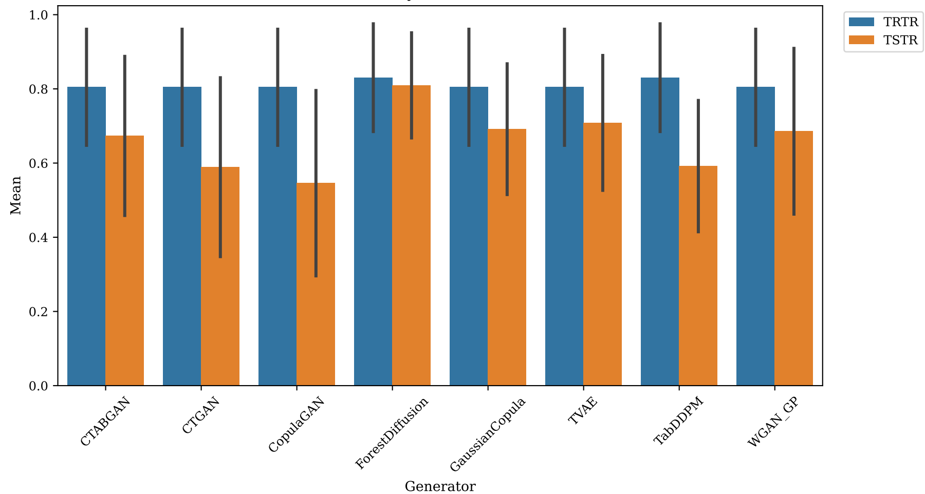
Accuracy: TRTR vs TSTR
