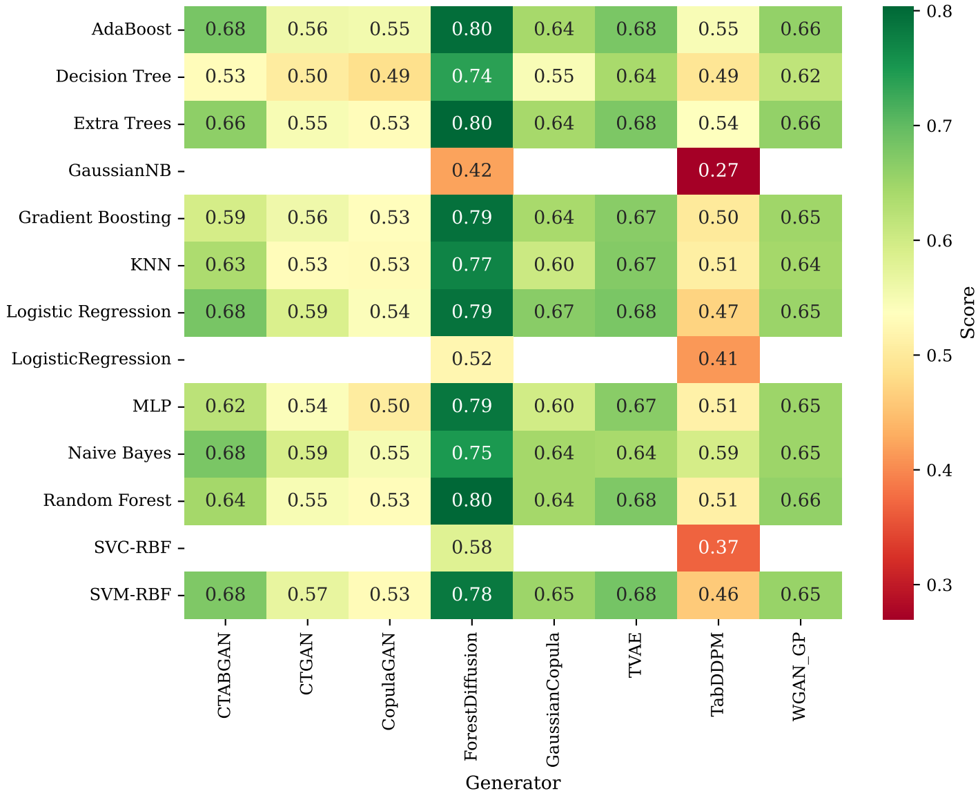
Classifier × Generator TSTR Heatmap
