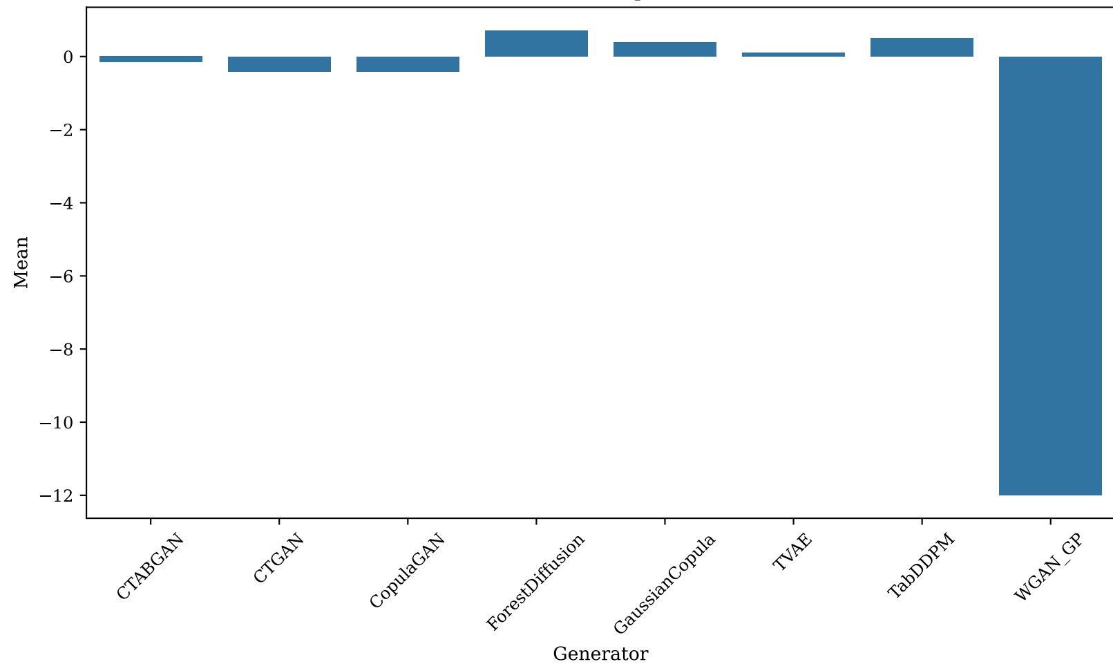
R2 TSTR Comparison
