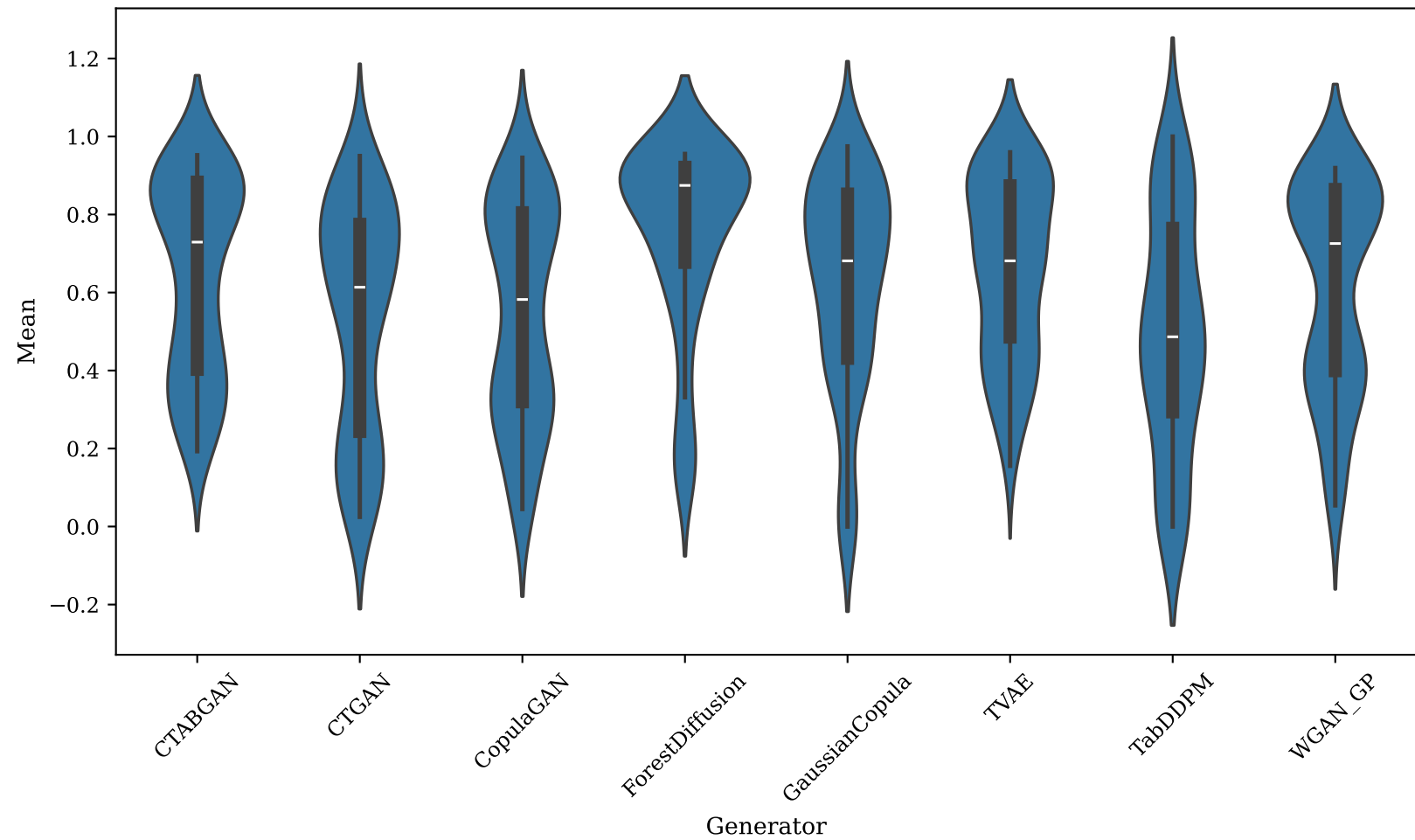
Recall TSTR Violin
