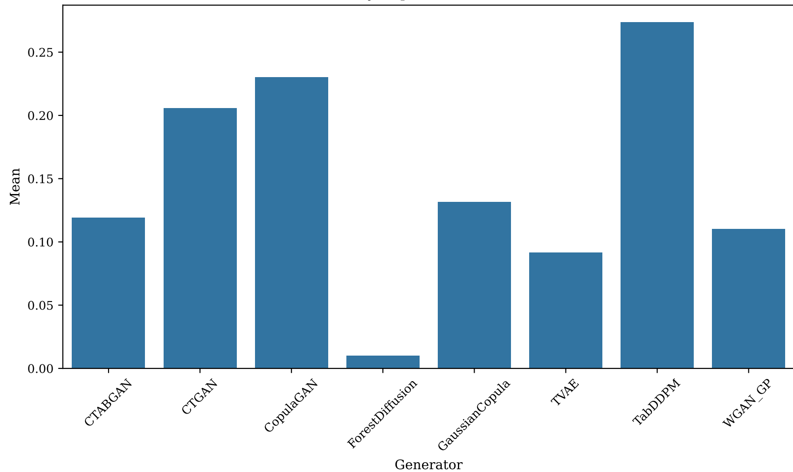
Utility Gap (TRTR – TSTR)
