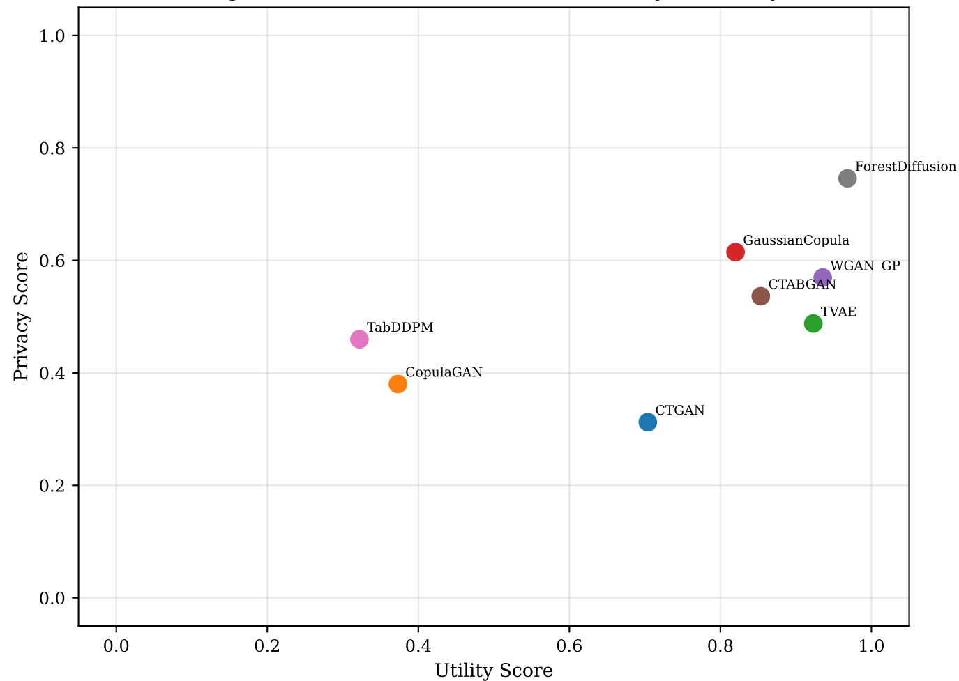
Figure 1: Wisconsin Breast Cancer — Utility Vs Privacy
