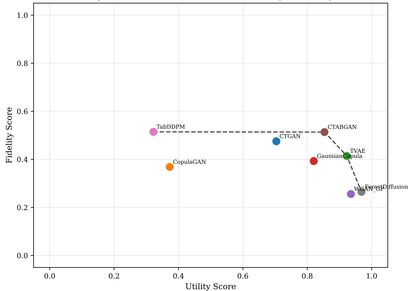
Figure 2: Wisconsin Breast Cancer — Utility Vs Fidelity
