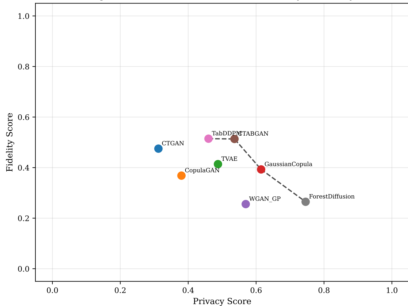
Figure 3: Wisconsin Breast Cancer — Privacy Vs Fidelity
