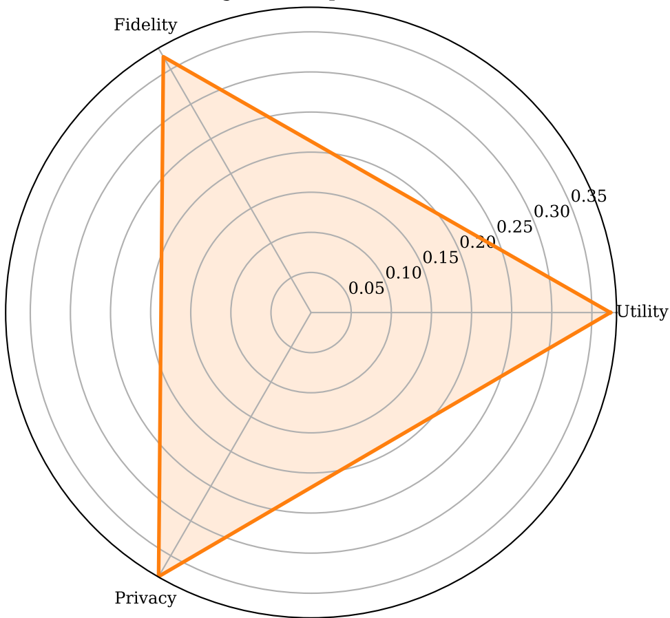
Figure 5: CopulaGAN
