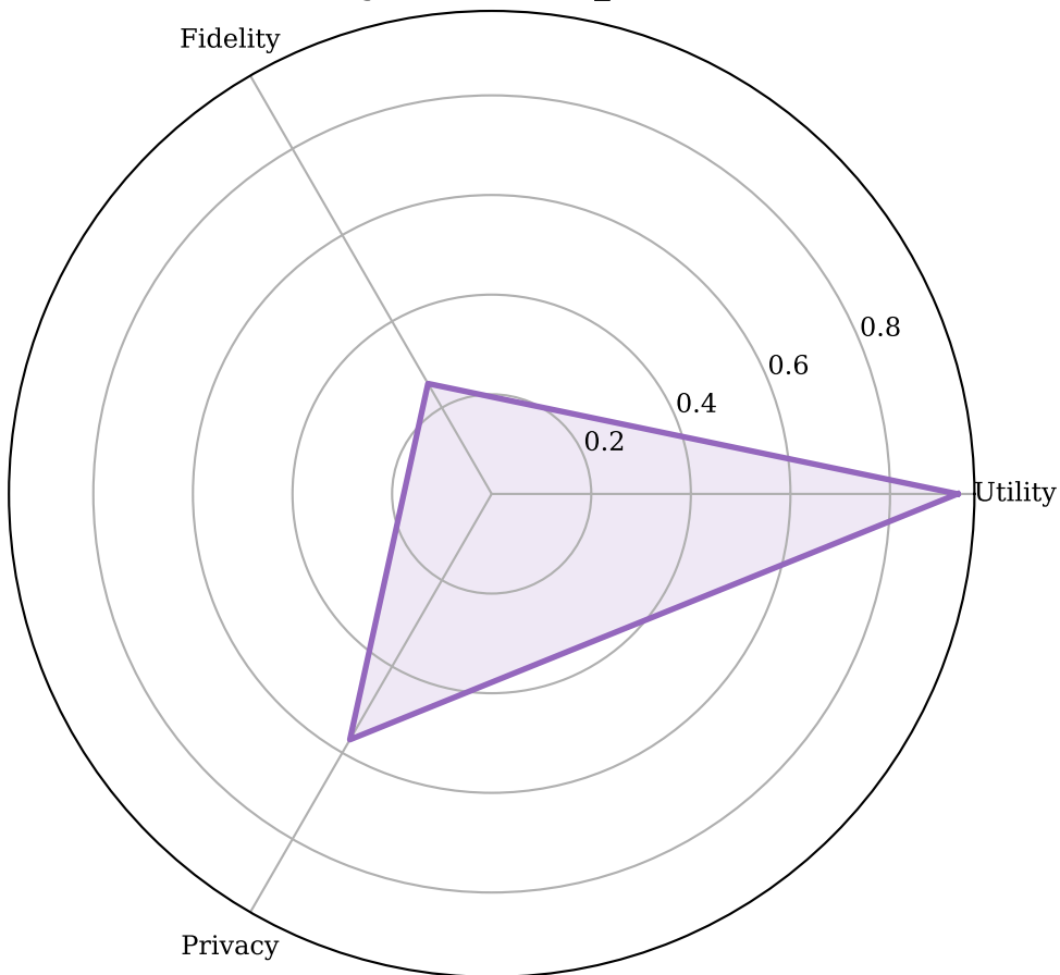
Figure 5: WGAN_GP
