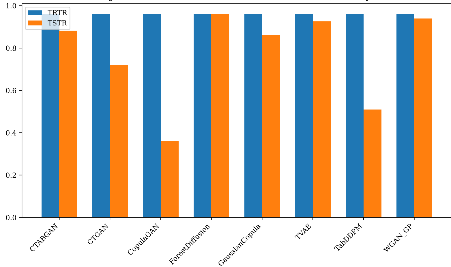
Figure 8: Wisconsin Breast Cancer — TRTR vs TSTR (Accuracy)
