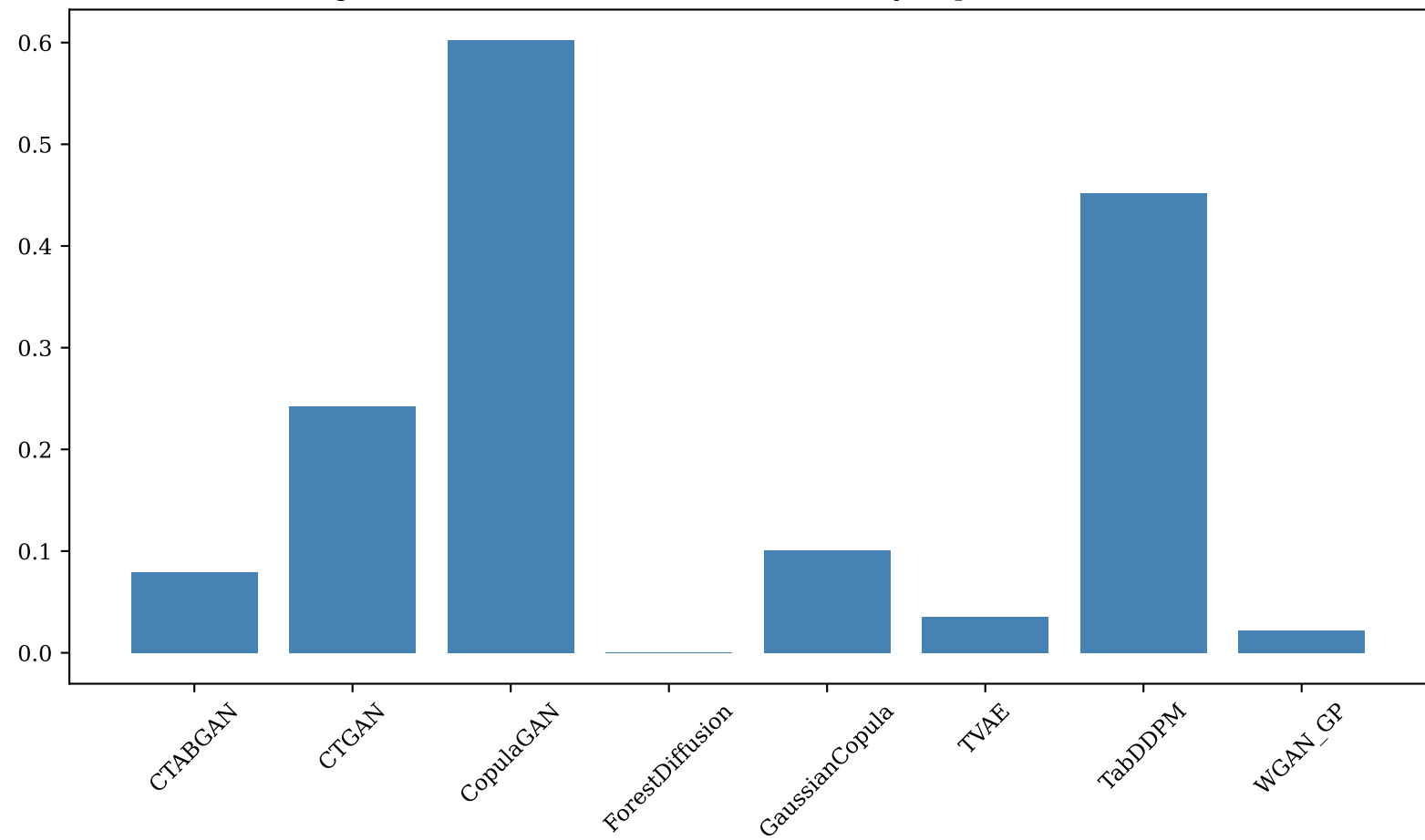
Figure 8: Wisconsin Breast Cancer — Utility Gap (TRTR – TSTR)
