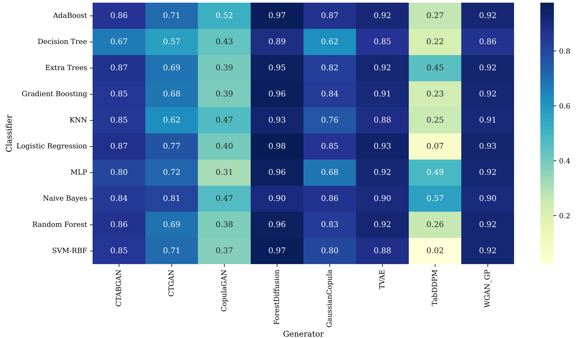
Figure 9: Wisconsin Breast Cancer — F1 by Classifier × Generator
