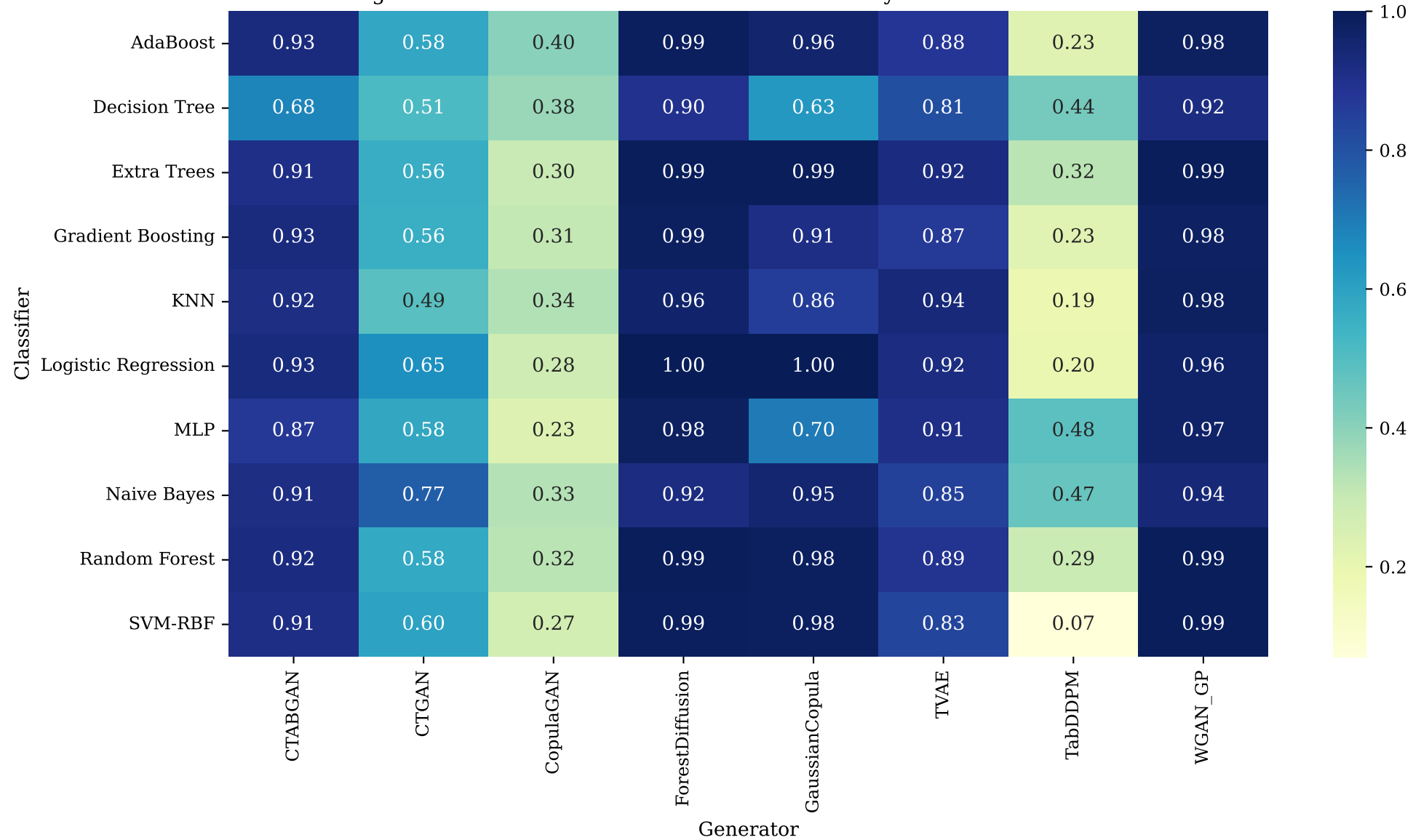
Figure 9: Wisconsin Breast Cancer — Precision by Classifier × Generator
