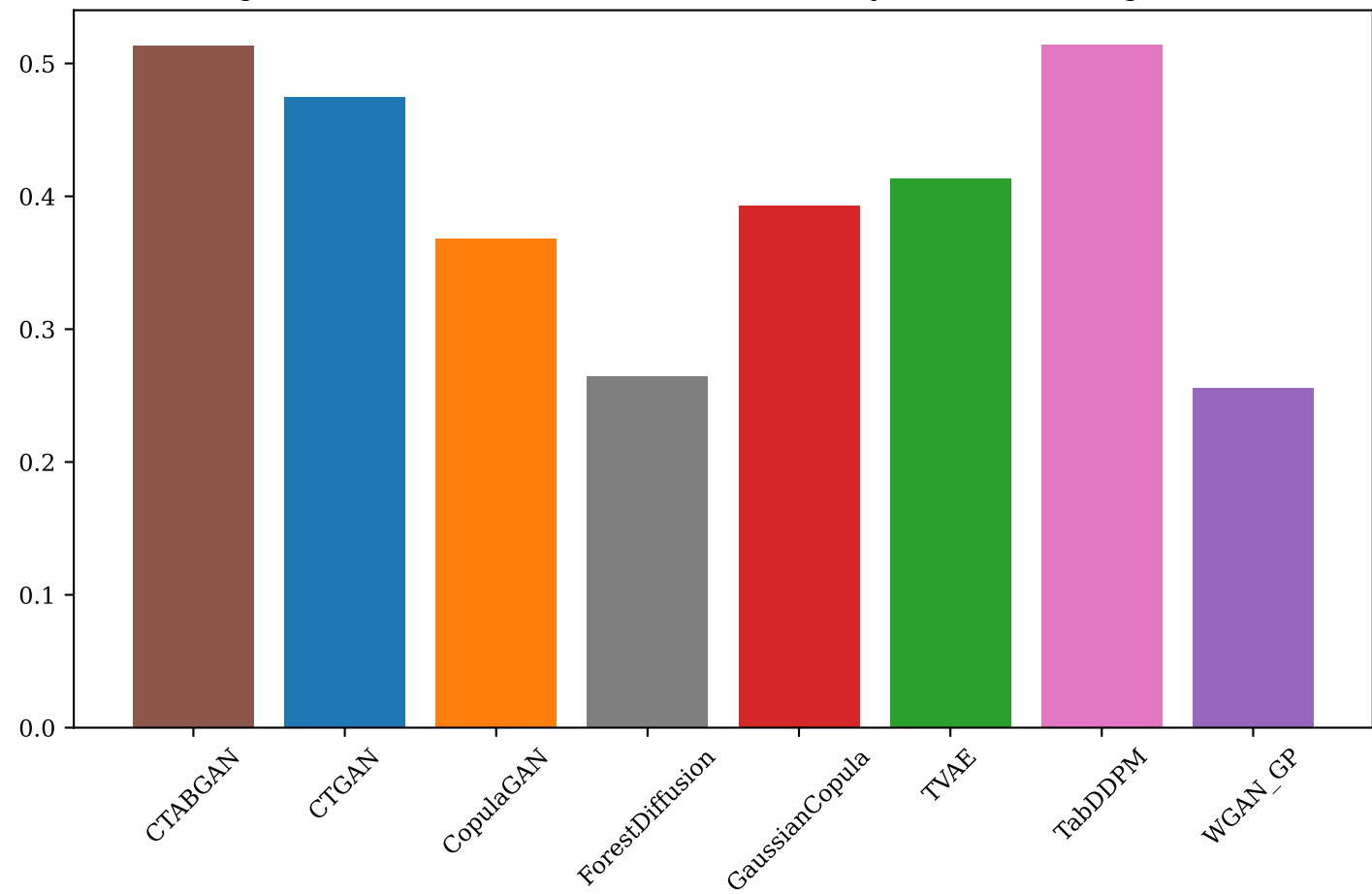
Figure 12: Wisconsin Breast Cancer — Fidelity (baseline Leakage=0%)
