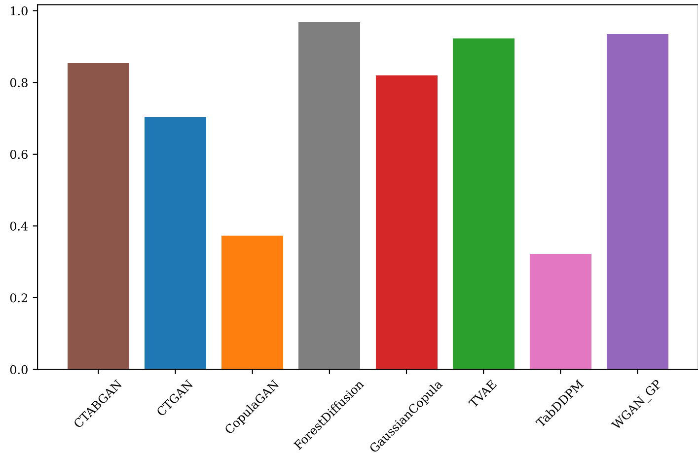
Figure 12: Wisconsin Breast Cancer — Utility (baseline Leakage=0%)
