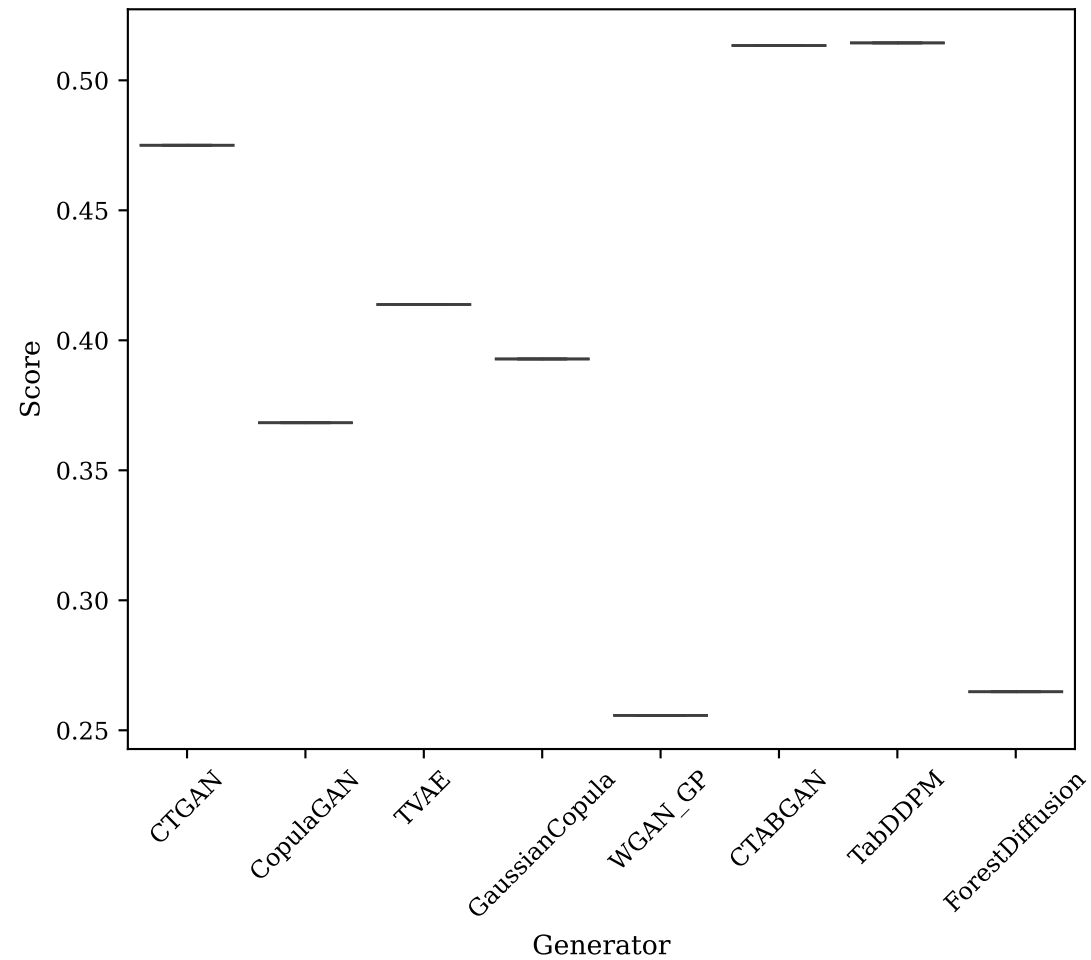
Fidelity Boxplot
