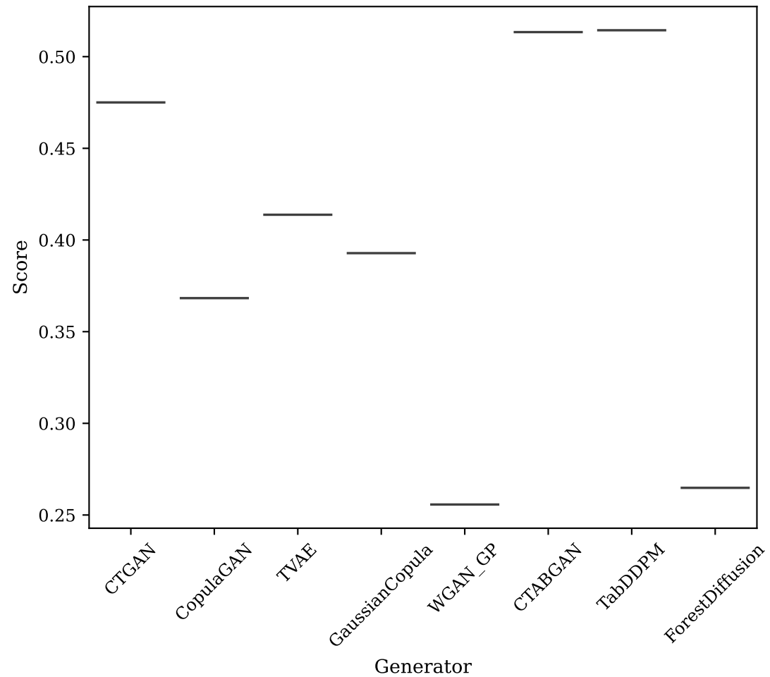
Fidelity Violin
