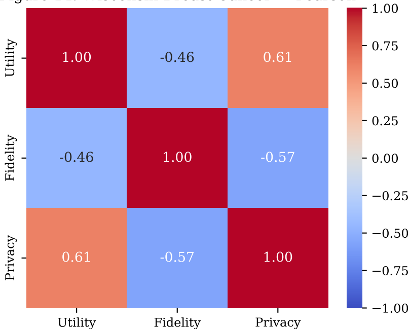
Figure 14: Wisconsin Breast Cancer — Pearson
