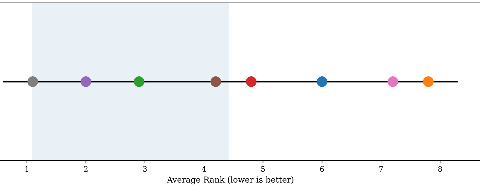
Figure 15: Wisconsin Breast Cancer — Critical Difference (Friedman + Nemenyi)
