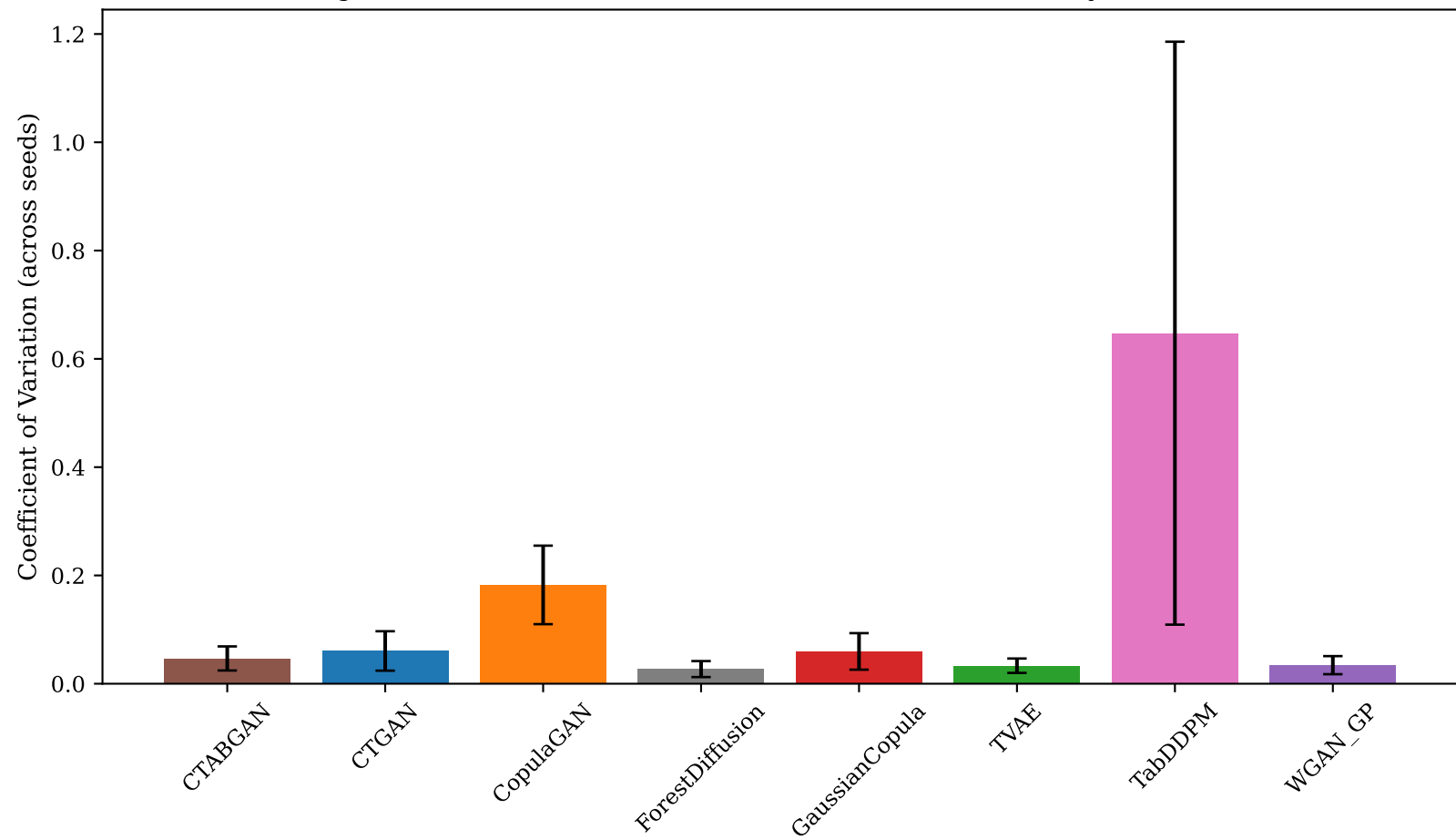
Figure 18: Wisconsin Breast Cancer — Generator Stability (10 seeds)
