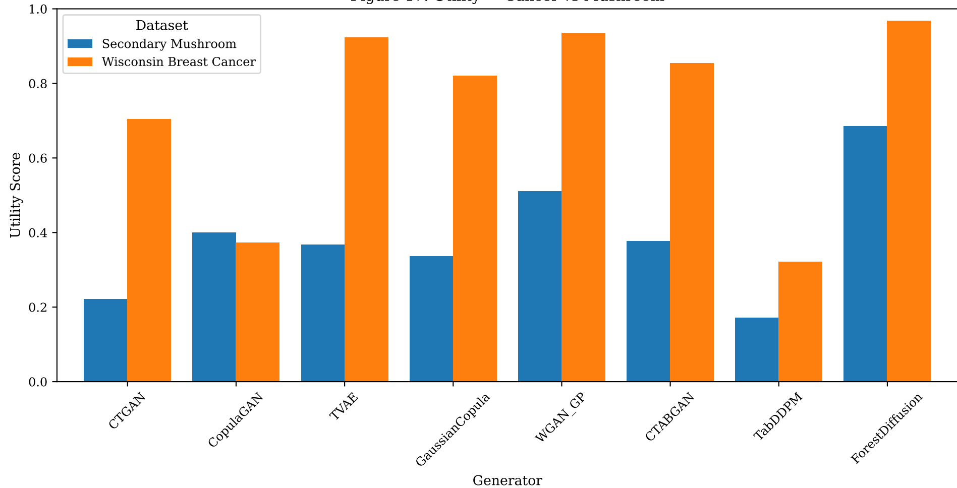
Figure 17: Utility — Cancer vs Mushroom
