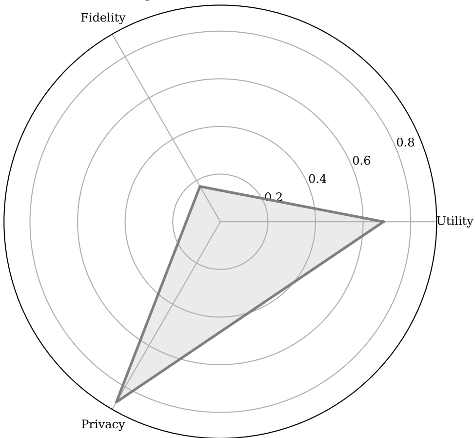
Figure 5: ForestDiffusion
