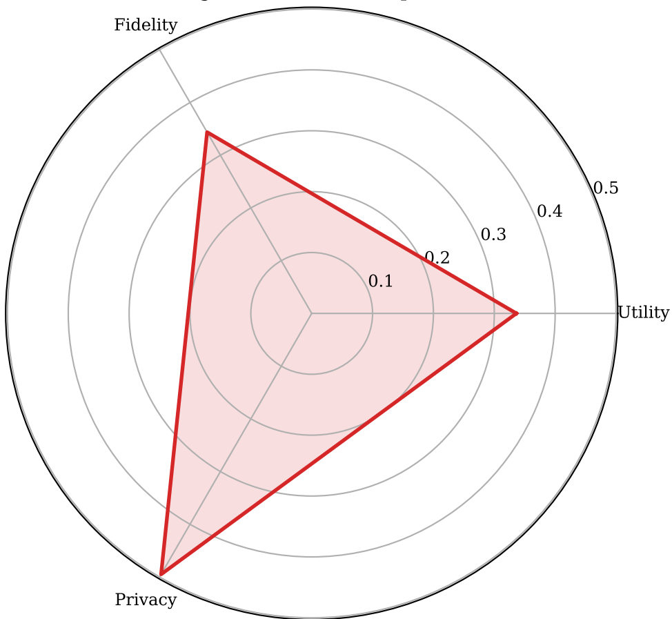
Figure 5: GaussianCopula
