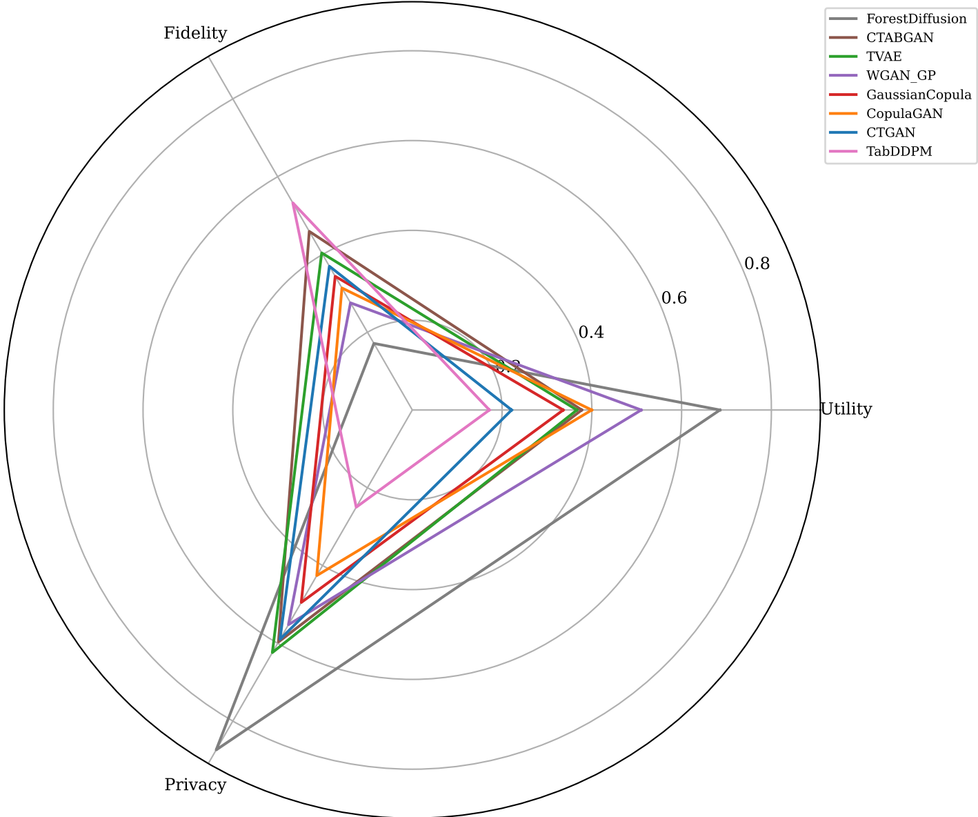
Figure 5: Secondary Mushroom — All Generators
