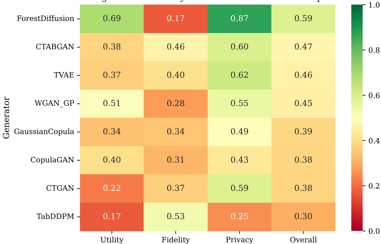
Figure 7: Secondary Mushroom — Score Heatmap
