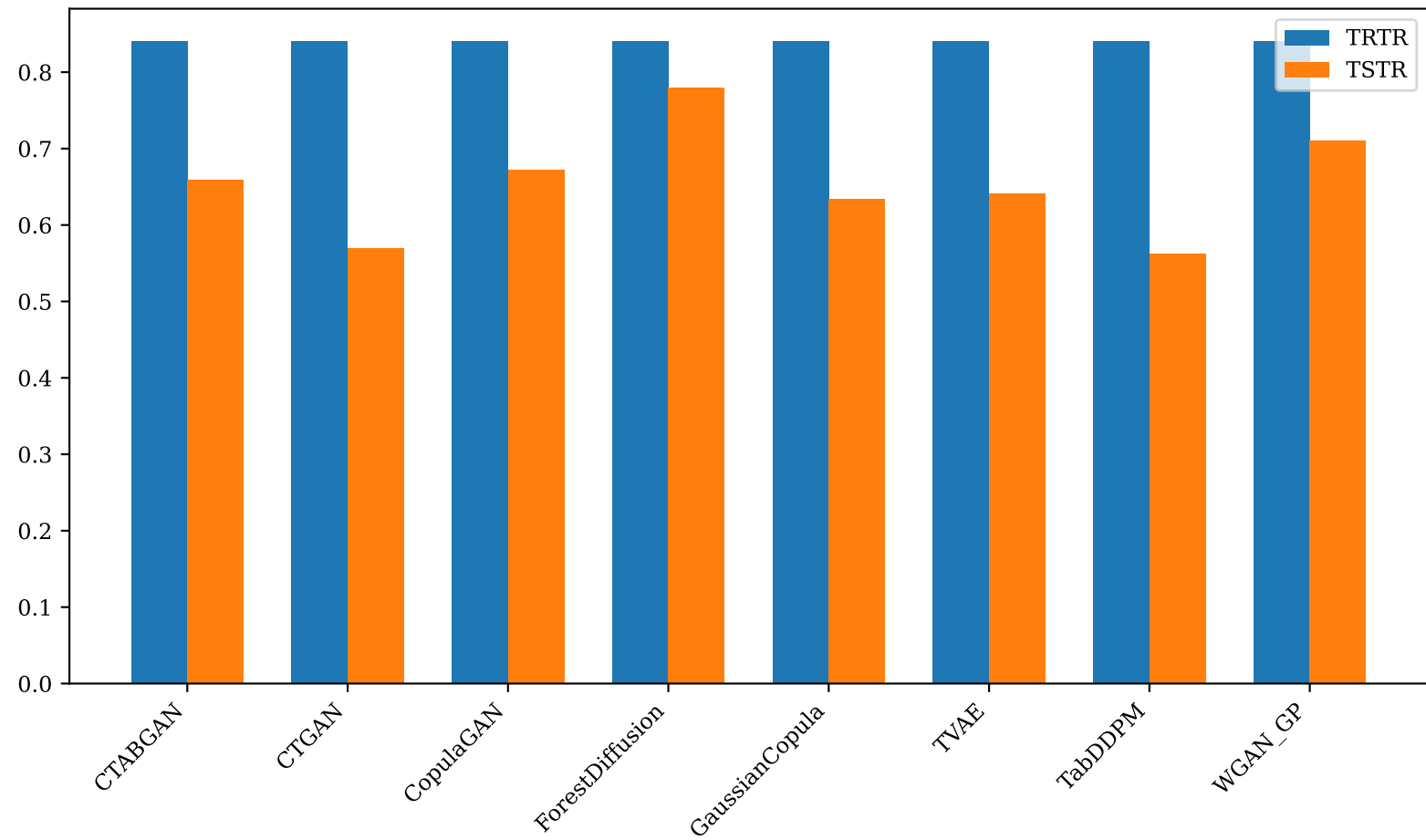
Figure 8: Secondary Mushroom — TRTR vs TSTR (F1)
