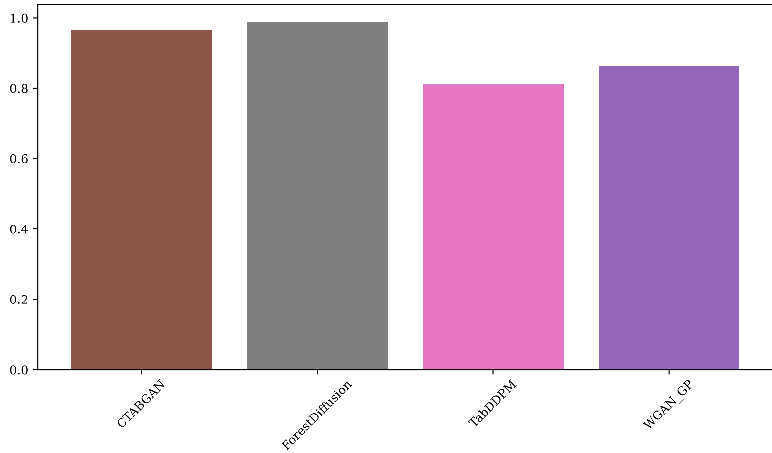
Figure 10: Secondary Mushroom — Hungarian_Cosine_Similarity
