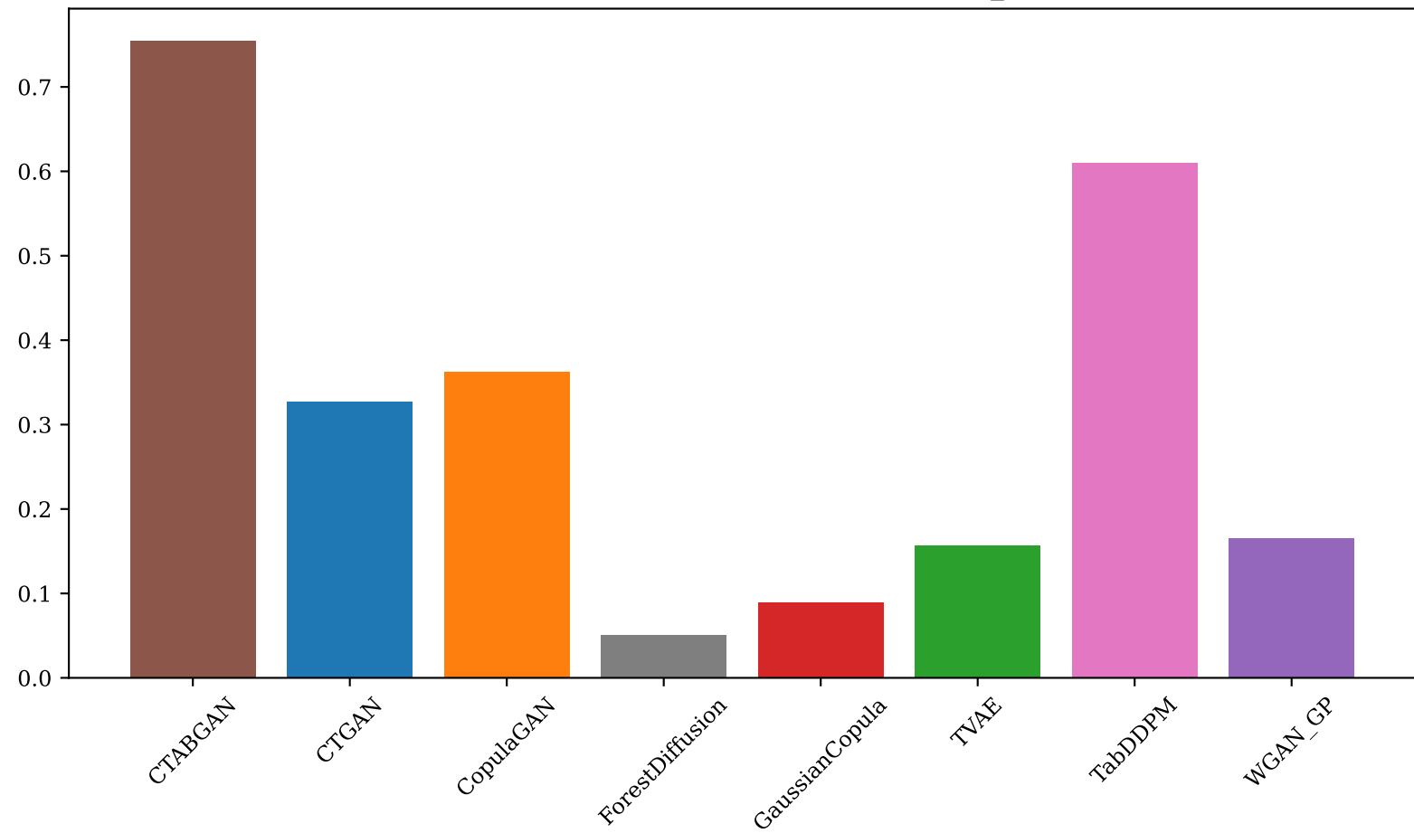
Figure 11: Secondary Mushroom — Correlation_Similarity
