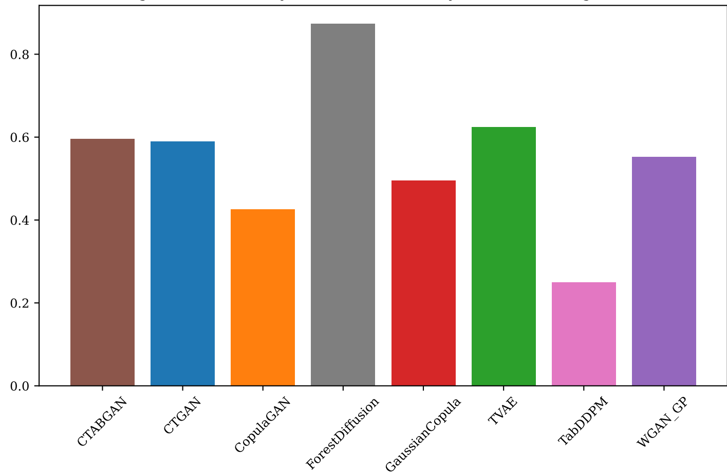
Figure 12: Secondary Mushroom — Privacy (baseline Leakage=0%)
