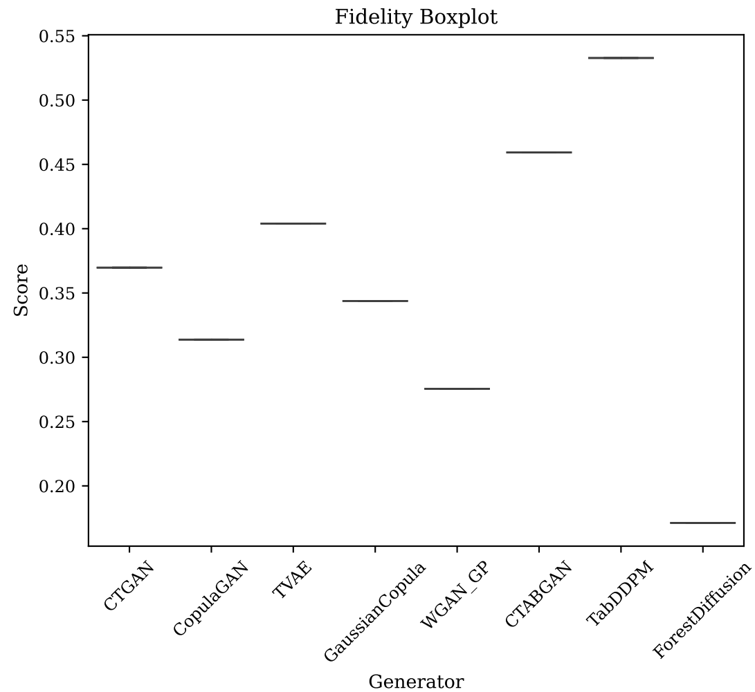
Figure 13: Secondary Mushroom — Fidelity Distribution
