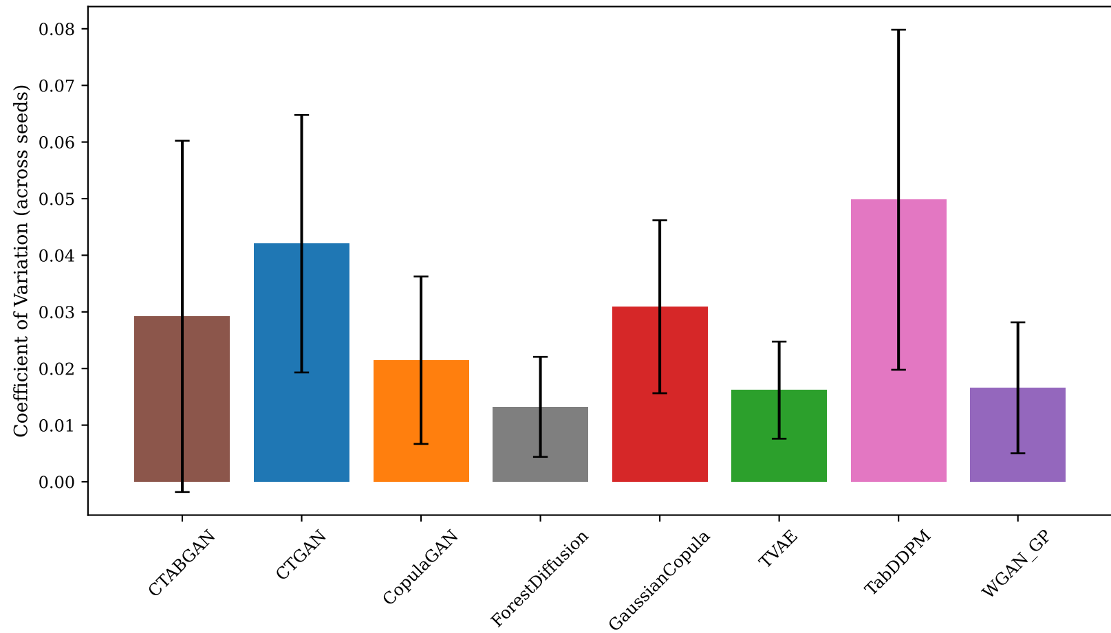
Figure 18: Secondary Mushroom — Generator Stability (10 seeds)
