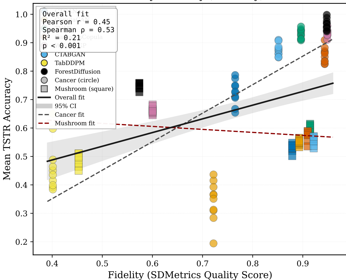
Fidelity vs Utility (Accuracy)
