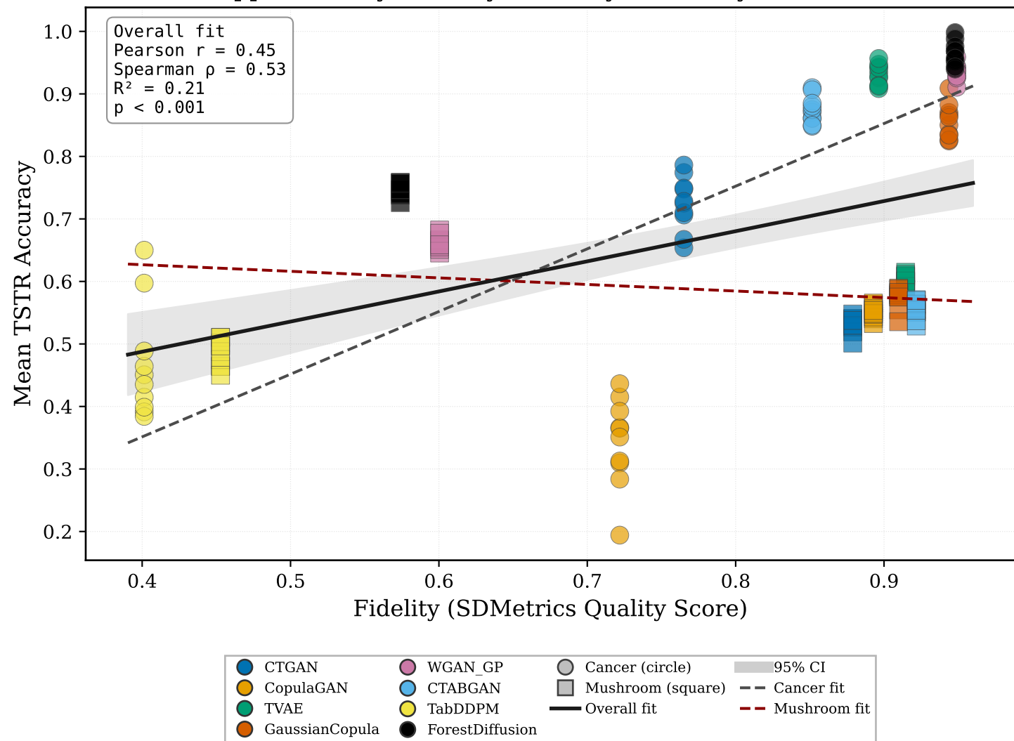
Supplementary: Fidelity vs Utility (Accuracy; seed-level)
