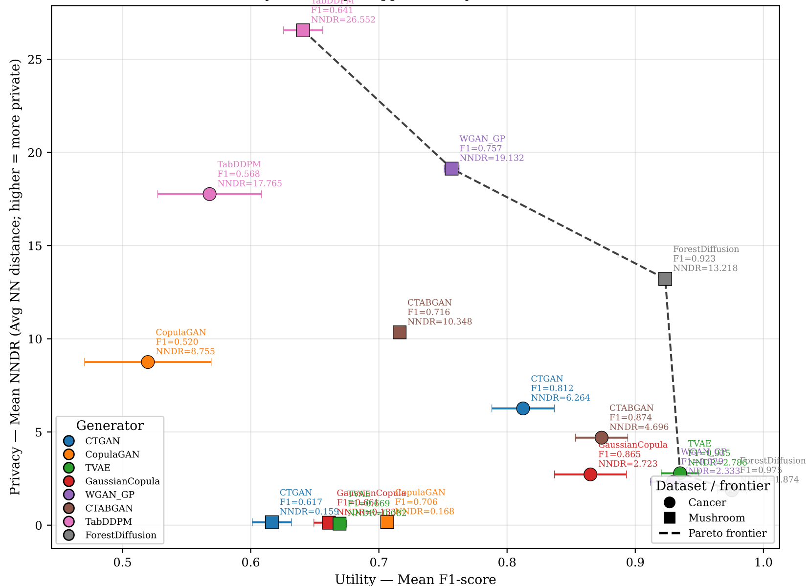
Utility vs Privacy (Supplementary — best classifier)
