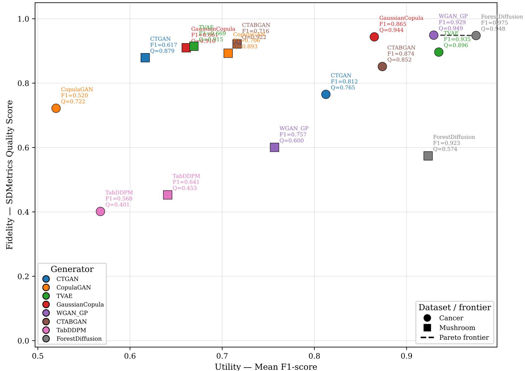
Utility vs Fidelity (Supplementary — best classifier)
