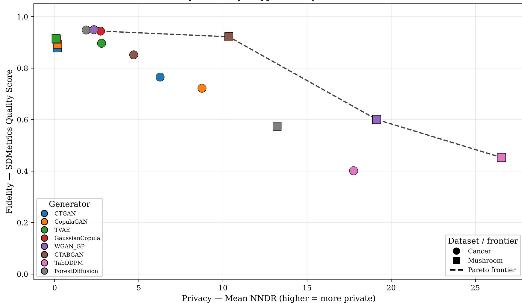
Privacy vs Fidelity (Supplementary — best classifier)
