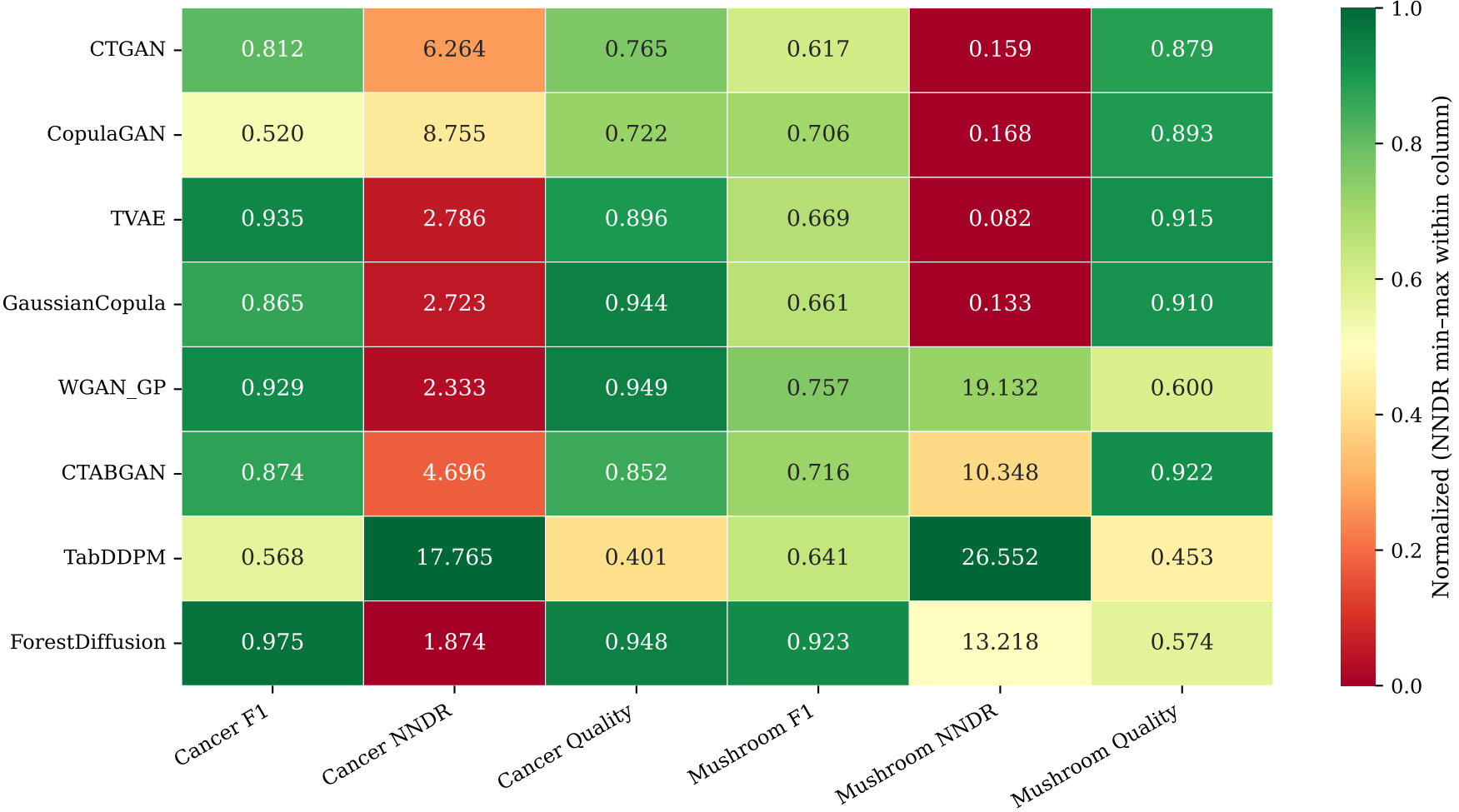
Heatmap — F1 / NNDR / Quality (Supplementary — best classifier)
