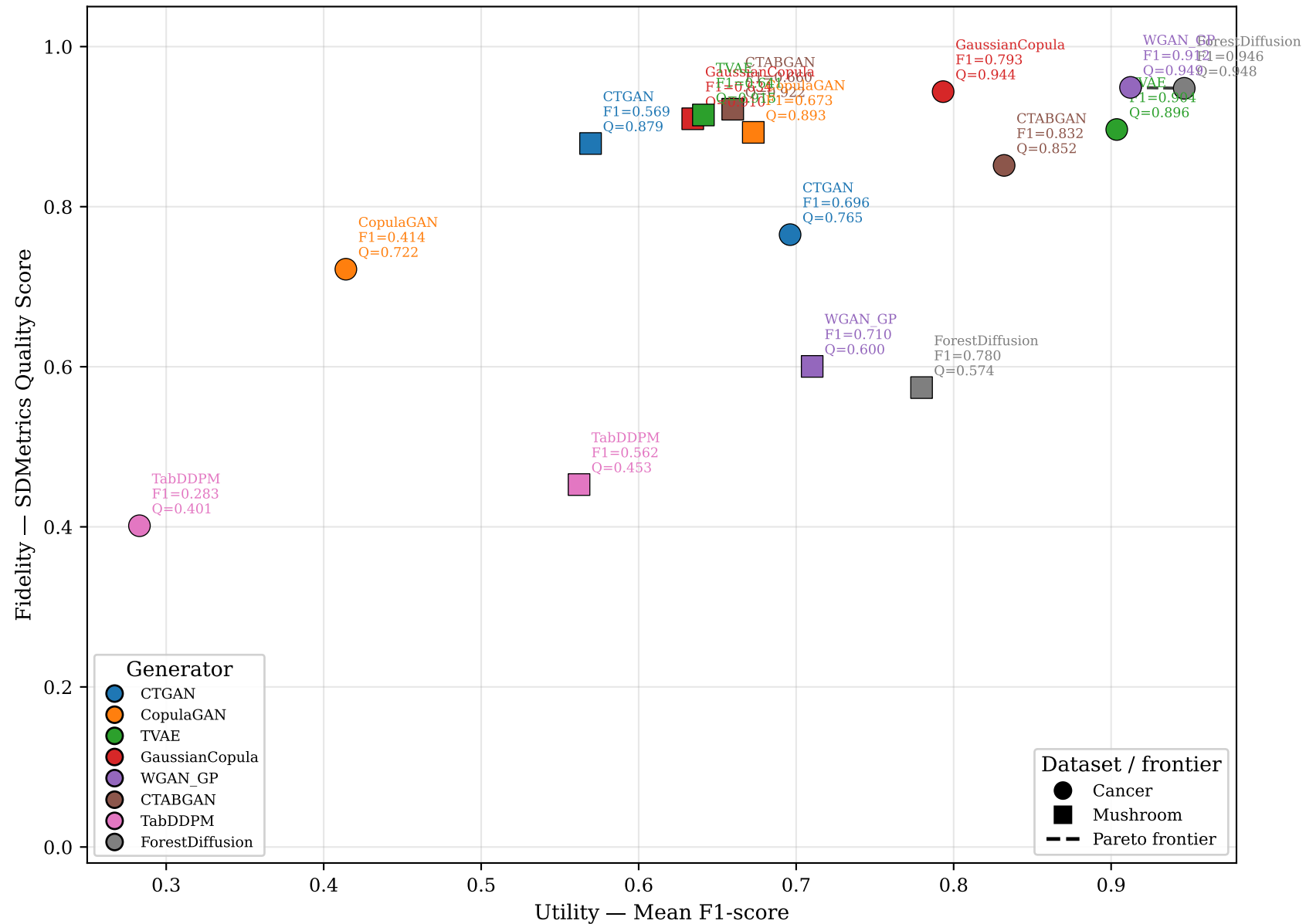
Utility vs Fidelity (Primary — classifier-independent)
