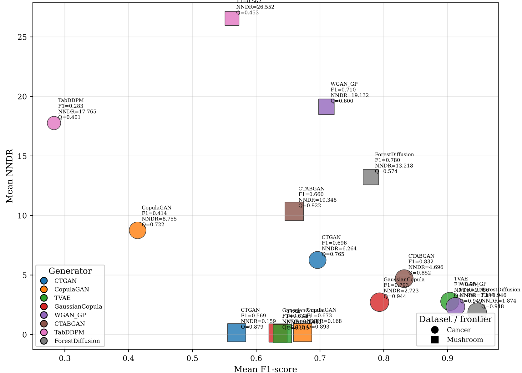
Bubble Trade-off (size = Quality) (Primary — classifier-independent)
