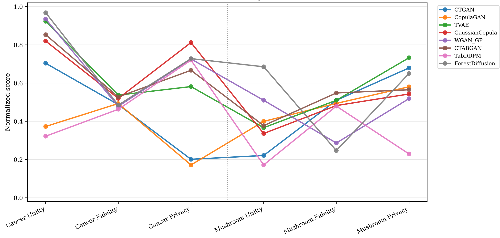
Parallel Coordinates — Consistency across Datasets
