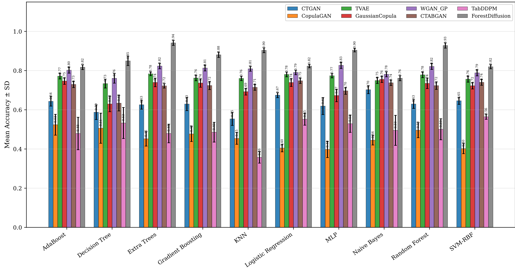
Classifier Comparison — Mean Accuracy by Generator (Cancer+Mushroom avg)
