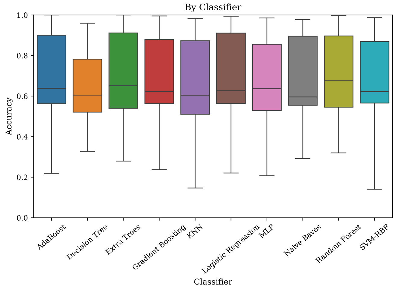
Accuracy Distributions (approx. from Mean \pm SD across 10 seeds)
