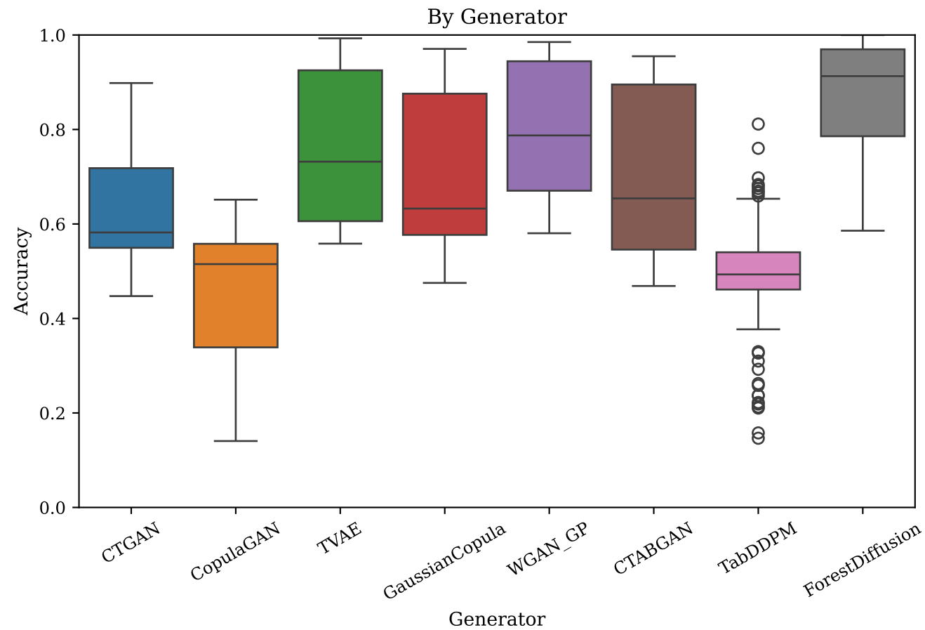
Accuracy Distributions (approx. from Mean \pm SD across 10 seeds)
