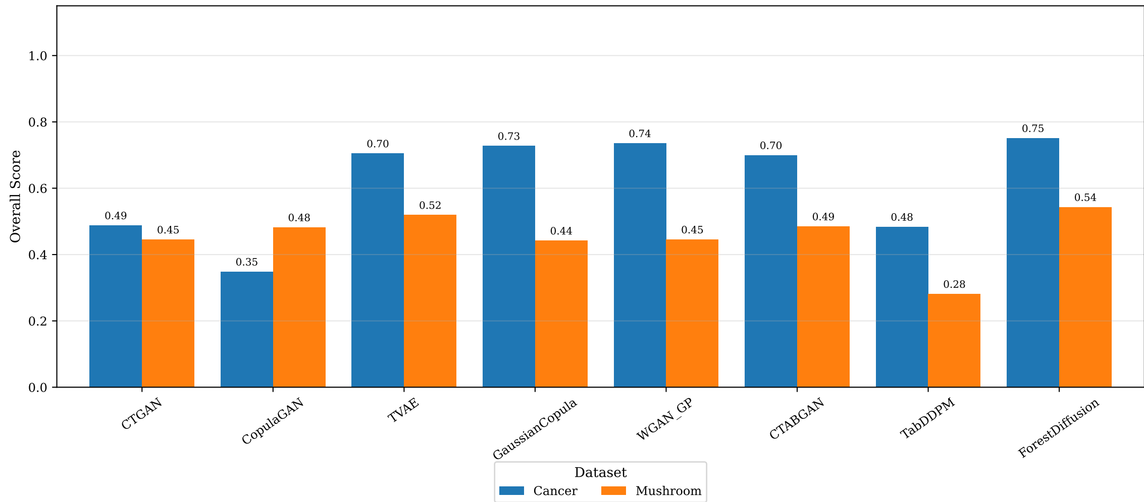
Overall — Cancer vs Mushroom
