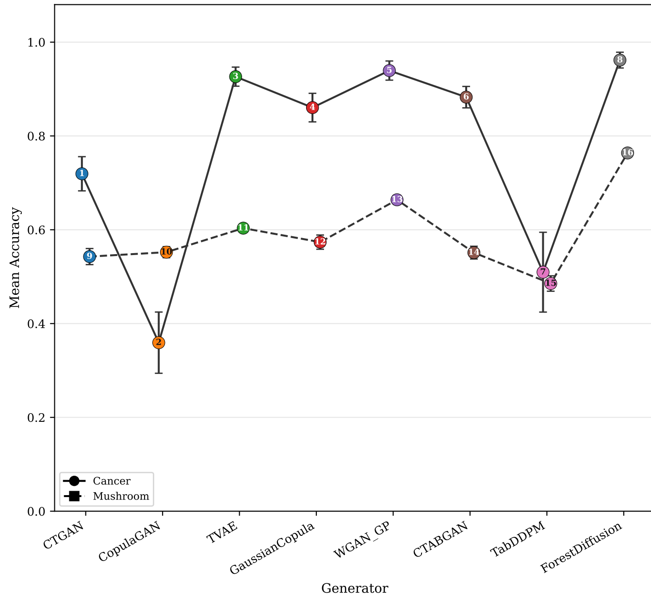
Mean Accuracy \pm SD (Leakage = 0% only)
