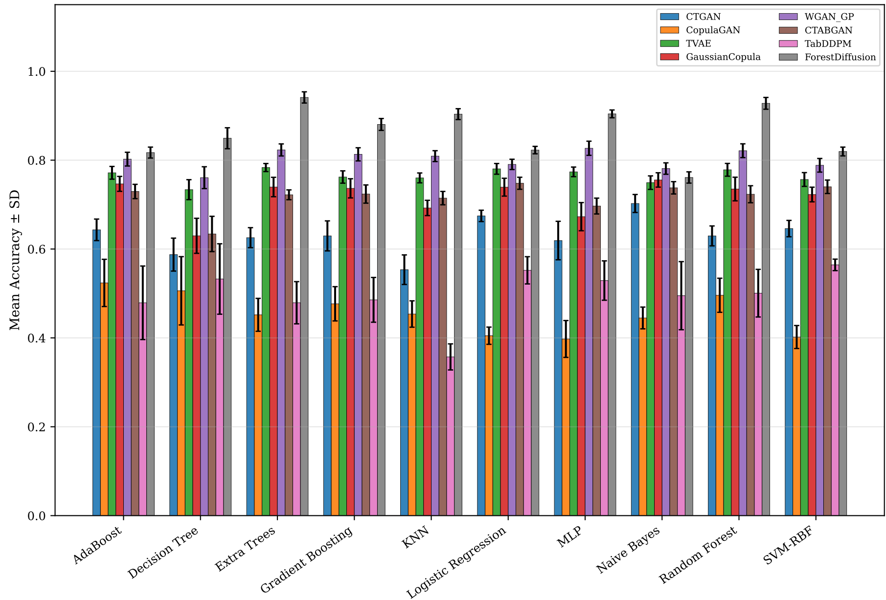
Classifier Comparison — Mean Accuracy by Generator (Cancer+Mushroom avg)
